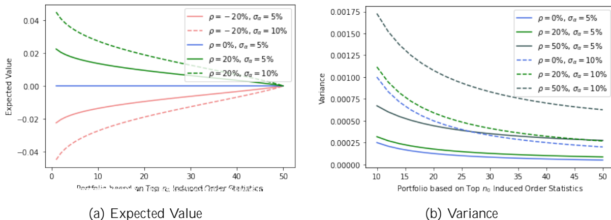
Figure A.2: Distribution of portfolio excess return formed by the top n_0 securities ranked by the impact factor, \mathbf{X} . The number of total securities, N , is set to be 50.
